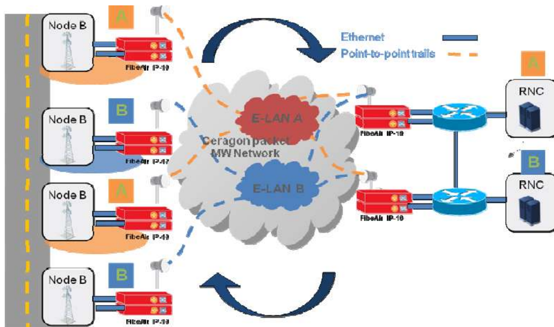
Figure 5: Full protected rural highway access backhaul
