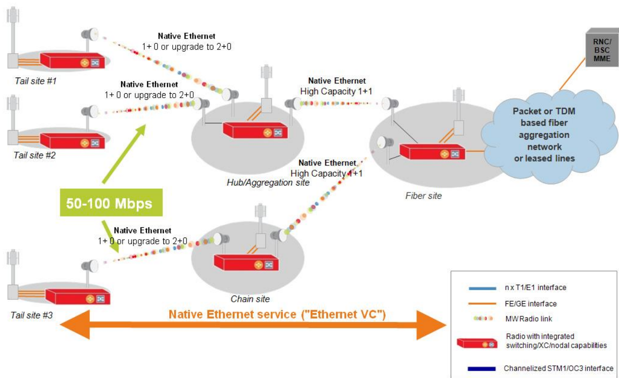
Figure 6: LTE – an All Packet network
