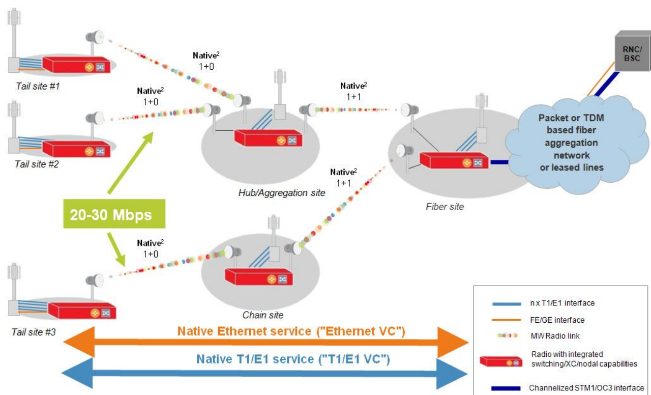
Figure 5: HSPA –TDM, ATM and Ethernet are supported
