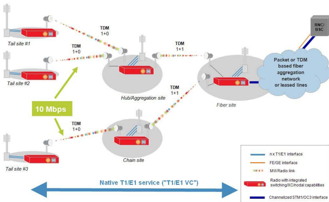
Figure 4: 2G/R99/R4 – TDM and ATM only
