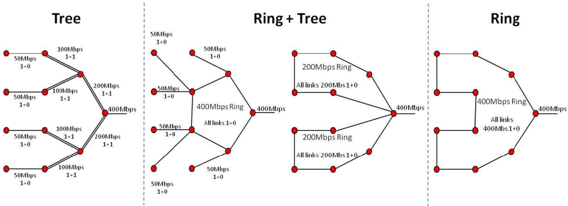
Figure 2: Examples of Aggregation Topologies
