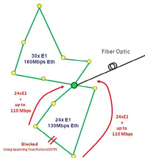
Figure 5: Doubling Ring Capacity using Spanning Tree Protocol
