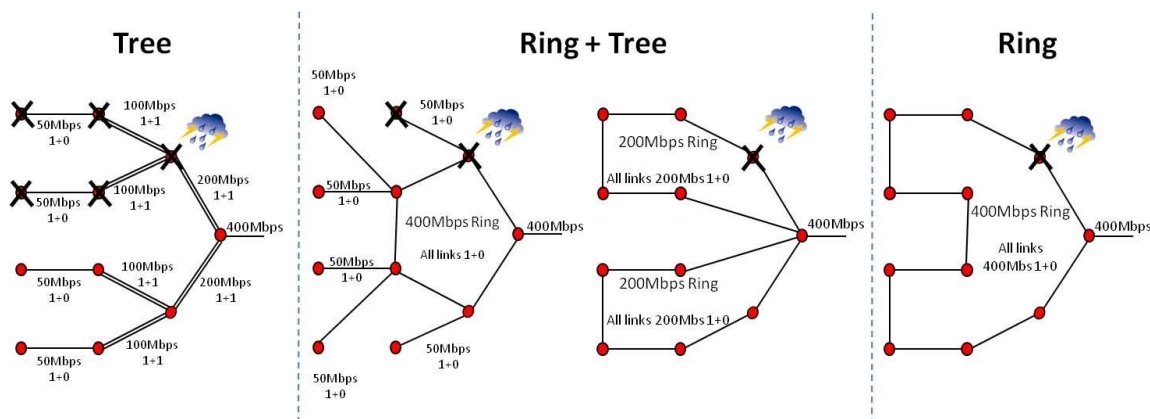
Figure 3: Protection Schemes in a Storm Scenario
