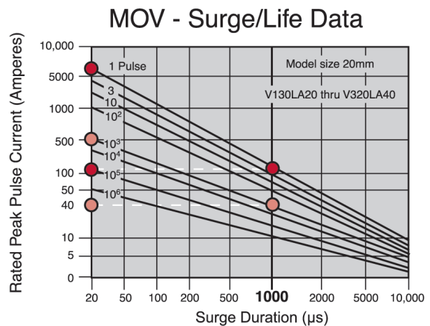
This graphic is republished from a MOV manufactures specification
